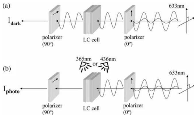
FIGURE 2 Schematic drawing of optical setup for transmittance measurement of LC cell.
