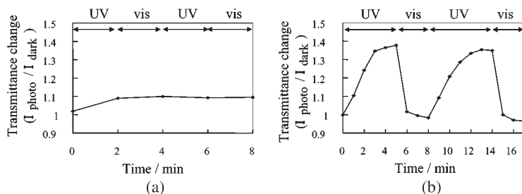
FIGURE 6 Transmittance changes at 633 nm by alternate exposure of UV and visible lights in LC cell constructed with hydrophobic 8AzO5 surface/5CB/hydrophobic 8AzO5 surface (a), and with hydrophilic 8AzO5 surface/5CB/hydrophobic 8AzO5 surface (b).
