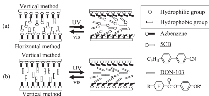
FIGURE 7 Schematic drawing of LC alignment change induced by photoisomerization of azobenzene in 5CB cell constructed with hydrophilic 8AzO5 surface/5CB/hydrophobic 8AzO5 surface (a), and in DON-103 cell constructed with hydrophobic 8AzO5 surface/DON-103/hydrophobic 8AzO5 surface (b).
